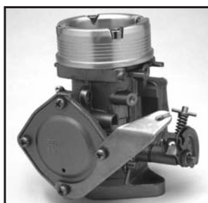
Diaphragm Cover Mount Throttle Cable Bracket 53-3313
