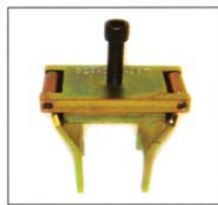
Drive Shaft / Floating Ring Part No. 950-102 O.E. No. 529-035-987 Fits: Super Charged 4-Tecs
